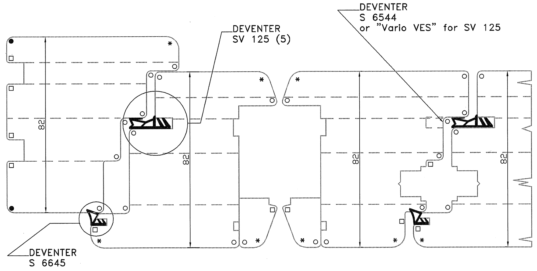
HORIZONTAL SECTION
