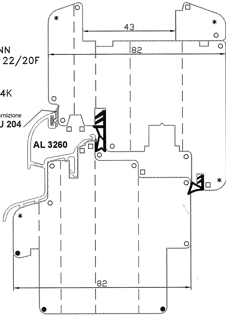
VERTICAL SECTION
