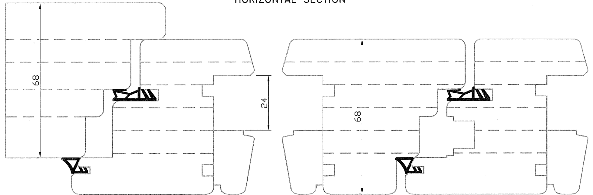
HORIZONTAL SECTION
